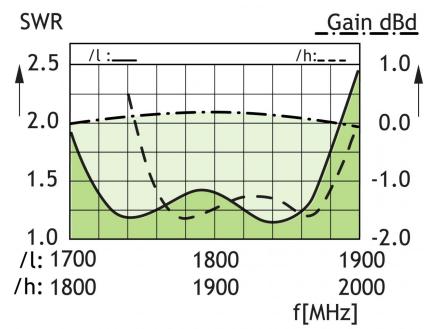
TYPICAL GAIN AND SWR CURVES
