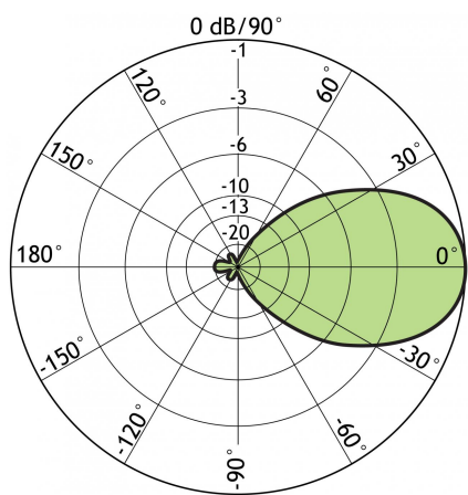
TYPICAL PATTERN (E-PLANE)
