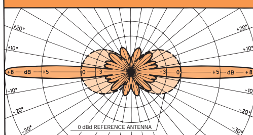
TYPICAL RADIATION PATTERN (E-PLANE)
