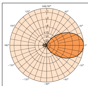
Outer ring: 6 dBd
