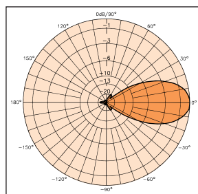
Outer ring: 11 dBd
